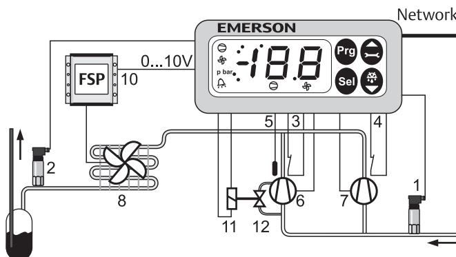
EC2-552 Condensing Unit Controller for 2 single stage compressors or 1 Digital Scroll™ and 1 single stage compressor
