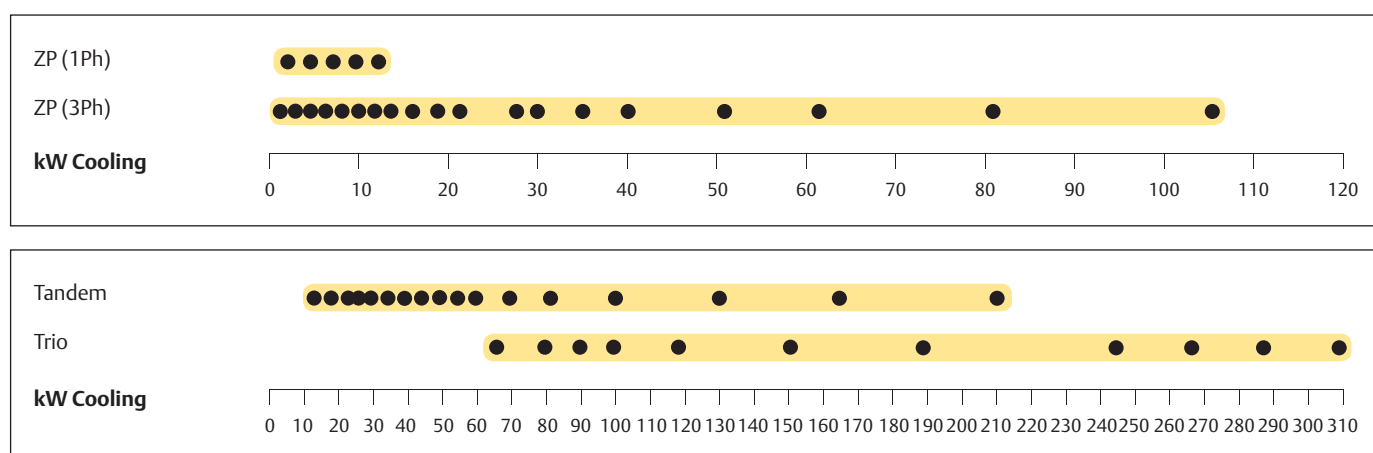
ZP Scroll Compressor
