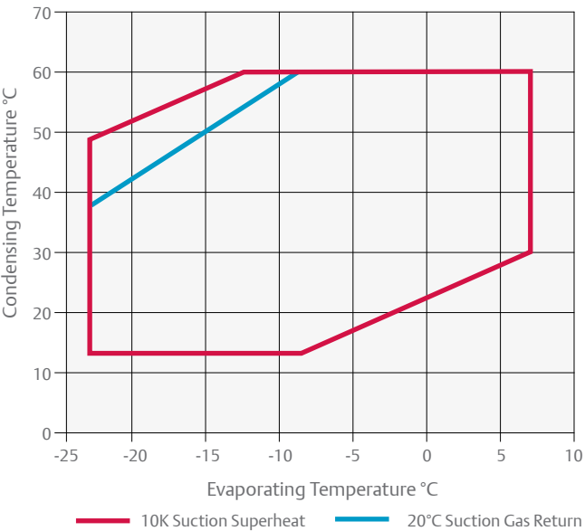
ZB*KA - R448A/R449A
