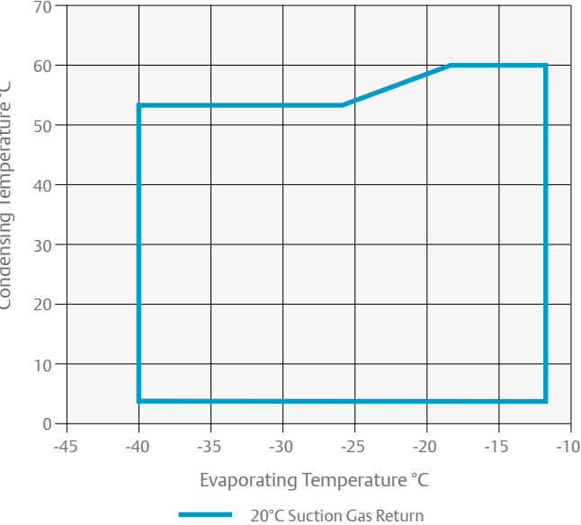
ZF*KA - R448A/R449A
