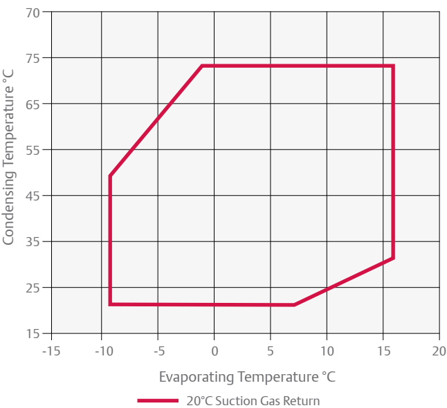
ZB*KA - R134a
